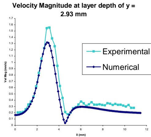
Figure 6. Velocity at y = 2.93 mm
