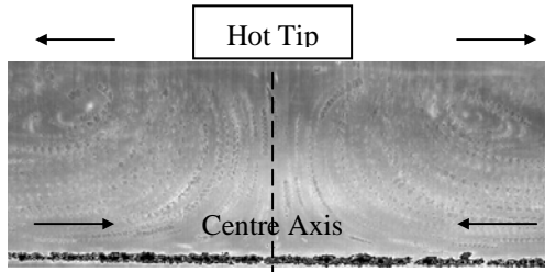
Figure 2. Flow patterns at the centre
